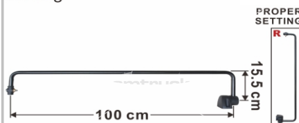
VV91-640R MIRROR ARM R=L
